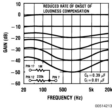
FIGURE 10. Loudness Compensated Volume Characteristic
