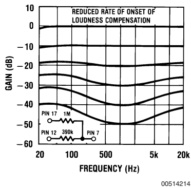
FIGURE 11. Loudness Compensated Volume Characteristic
