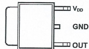
TO-252
